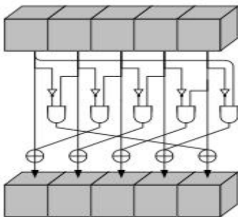
Figure 1: The Permuting Function introduced by Bertoni et al. [1], [2], [3], [4]
