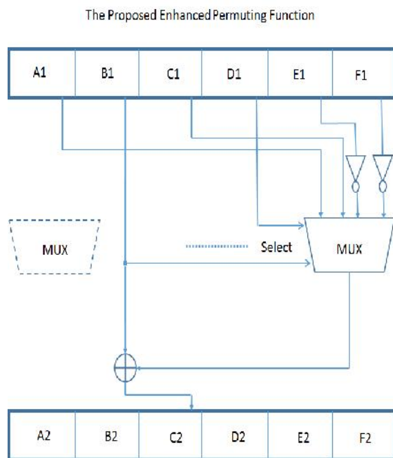
Figure 2 The Proposed Permuting Function
